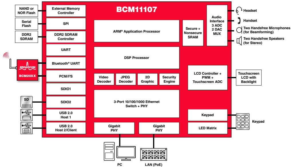
BCM1107 Block Diagram
